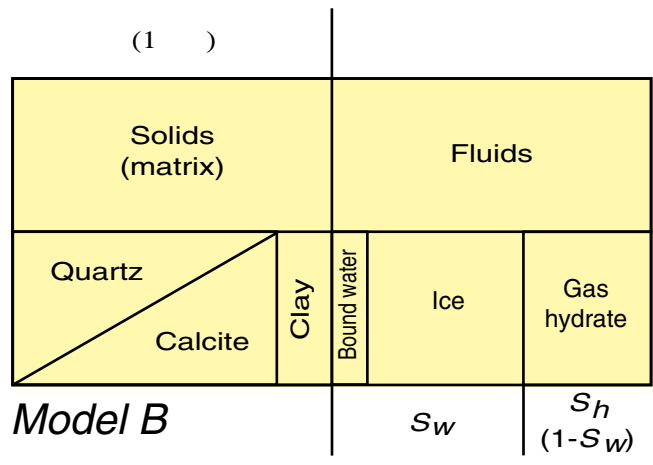
Figure 4b--Permafrost associated gas-hydrate reservoir model for conditions above the base of ice-bearing permafrost (Model B).
