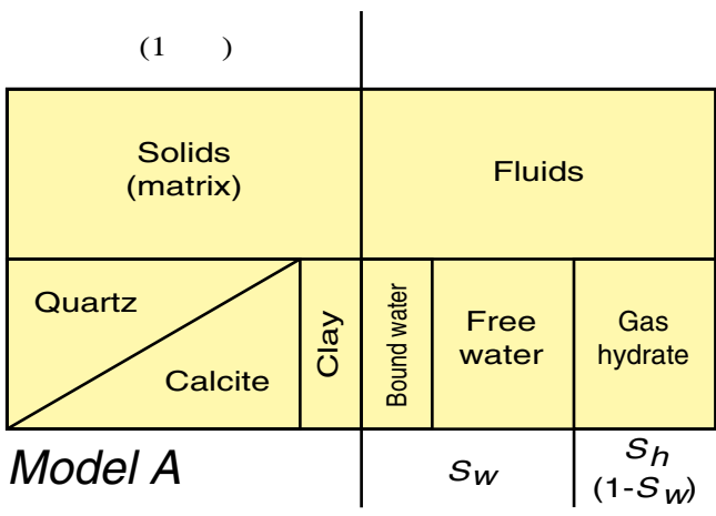
Figure 4a--Permafrost associated gas-hydrate reservoir model for conditions below the base of ice-bearing permafrost (Model A).
