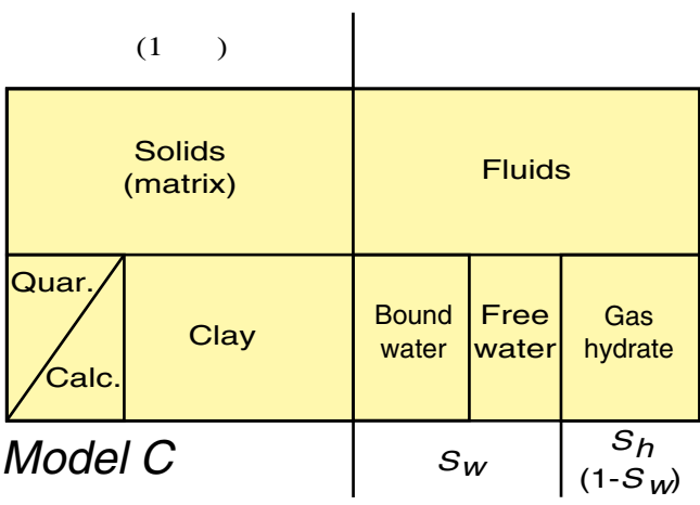
Figure 4c--Marine (clay-rich) gas-hydrate reservoir model (Model C).
