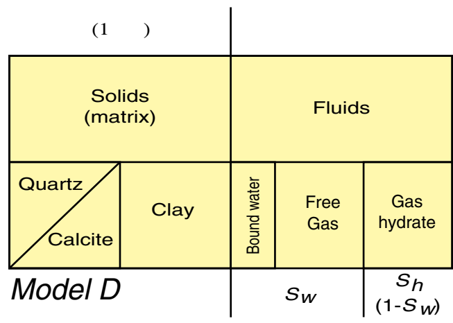
Figure 4d--Free-gas- and gas-hydrate-bearing reservoir model (Model D).
